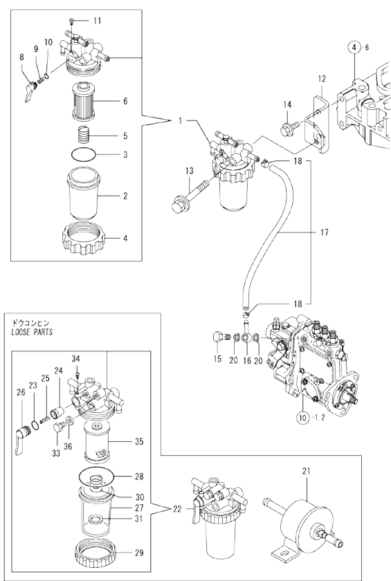
Fig.13. FUEL LINE
