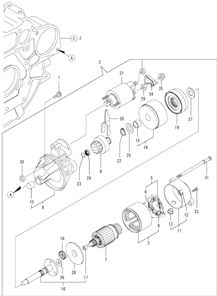
OCD10-M81601 3TNV76-SIK/QIK Fig.14. STARTING MOTOR
