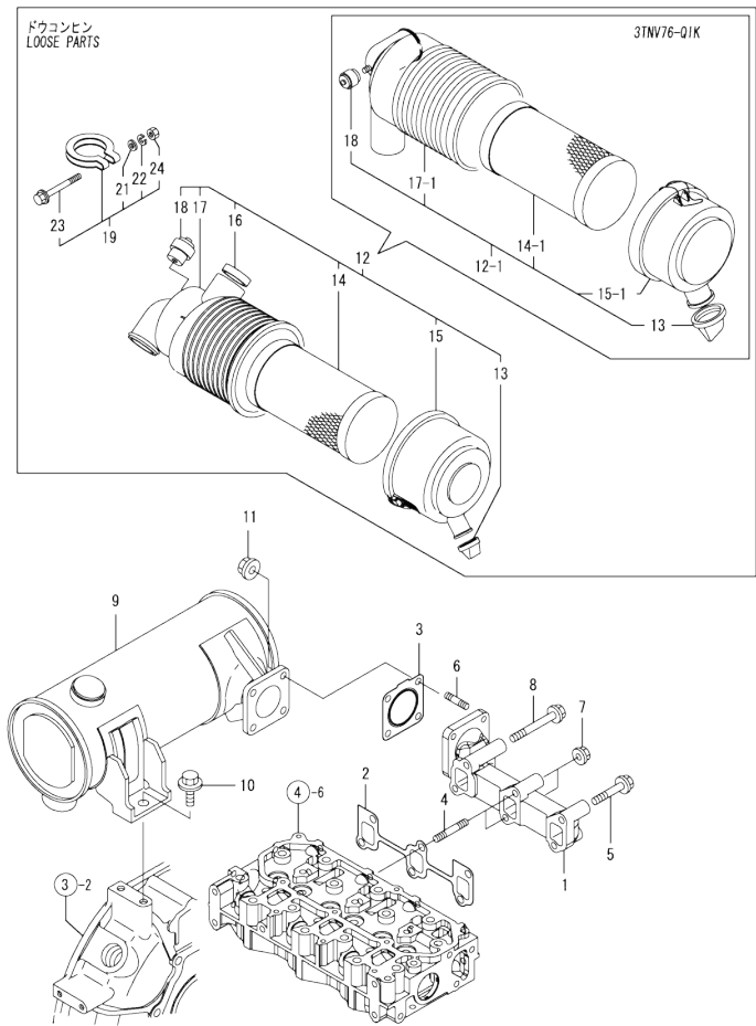
Fig.5. EXH. MANIFOLD, SILENCER & AIR CLEANER
