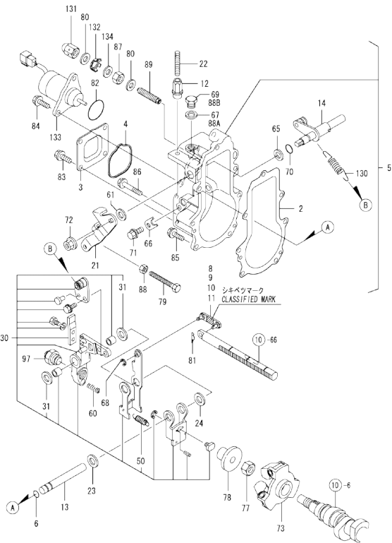
Fig.11. GOVERNOR
