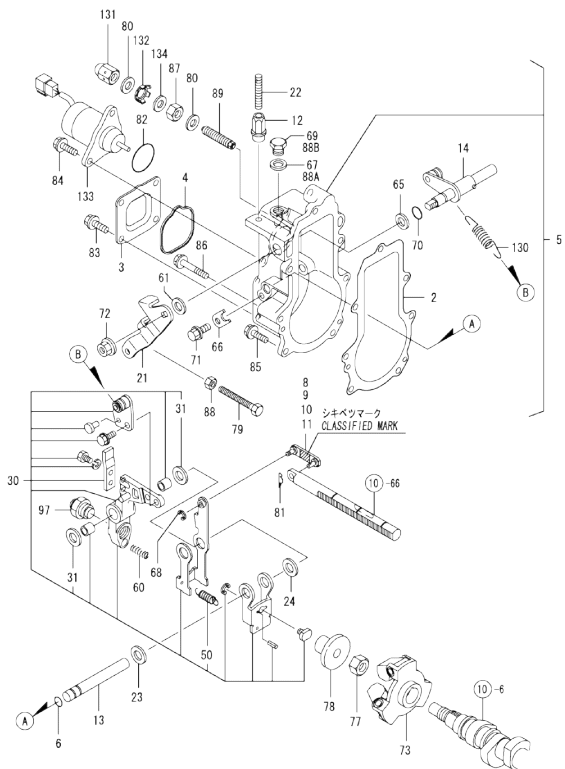
Fig.11. GOVERNOR
