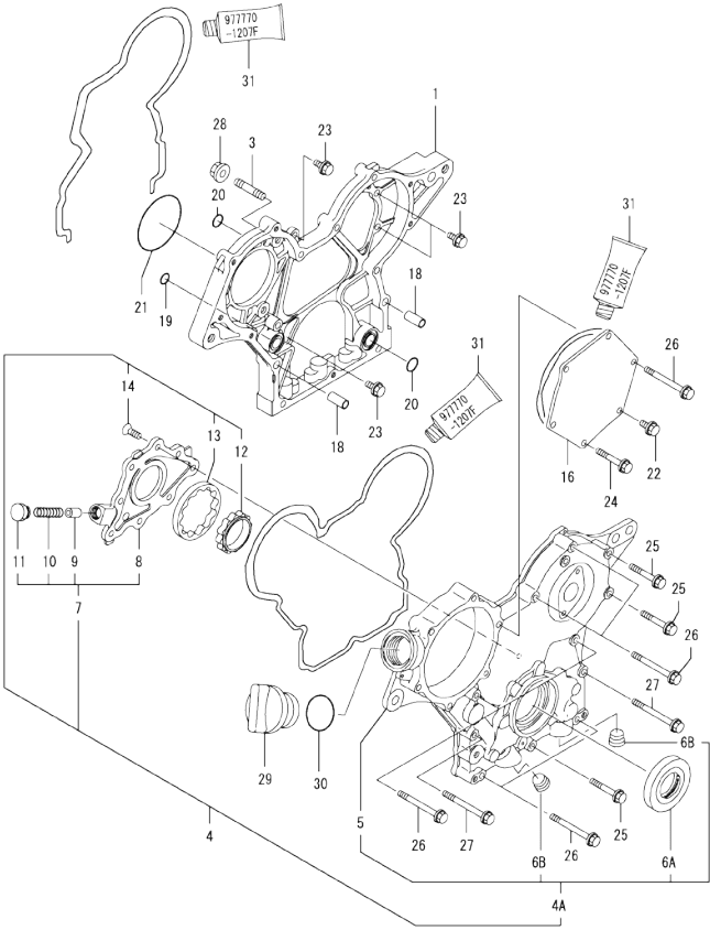
OCD10-M81601 3TNV76-SIK/QIK Fig.2. GEAR HOUSING
