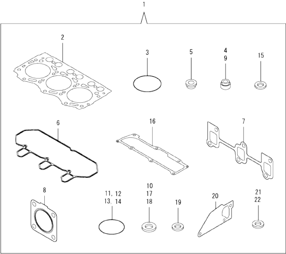
OCD10-M81601 3TNV76-SIK/QIK Fig.16. GASKET SET
