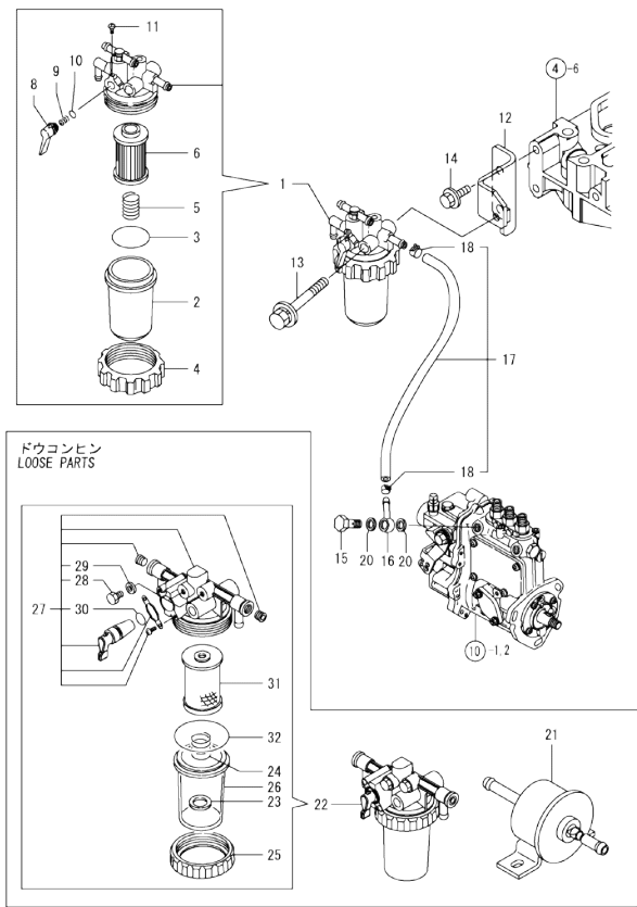
Fig.17. (13A)FUEL LINE
