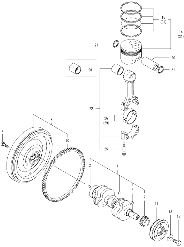
Fig.7. CRANKSHAFT & PISTON
