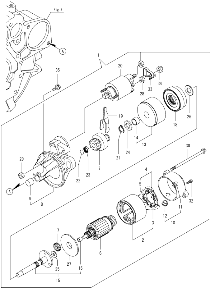
Fig.14. STARTER MOTOR
