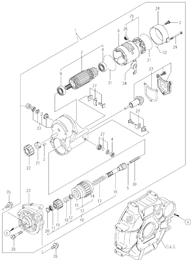
OCD50-M00260 3TNV76-SSU Fig.15. STARTING MOTOR
