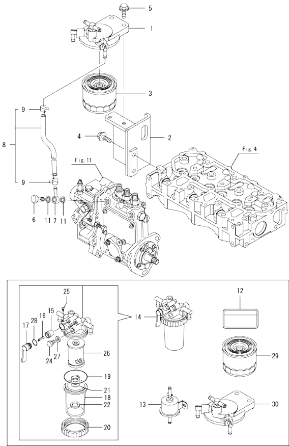
Fig.14. FUEL PIPE
