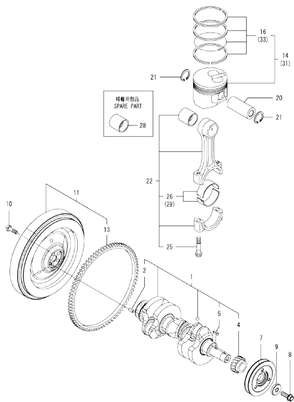
OCD50-M01760 3TNV76-SYBU Fig.7. CRANKSHAFT & PISTON
