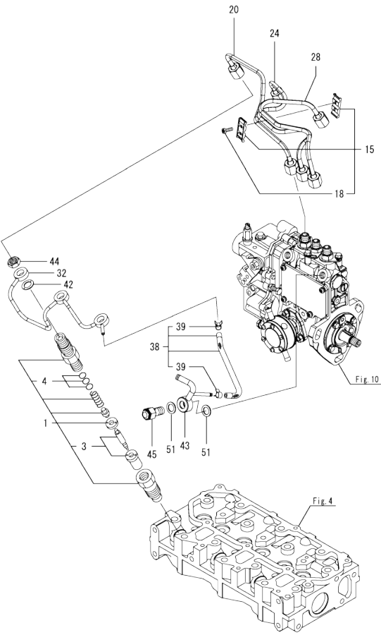
Fig.12. FUEL INJECTION VALVE
