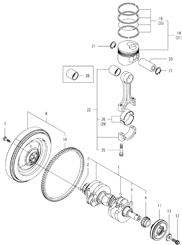
Fig.7. CRANKSHAFT & PISTON
