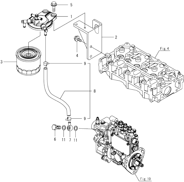
Fig.13. FUEL FILTER
