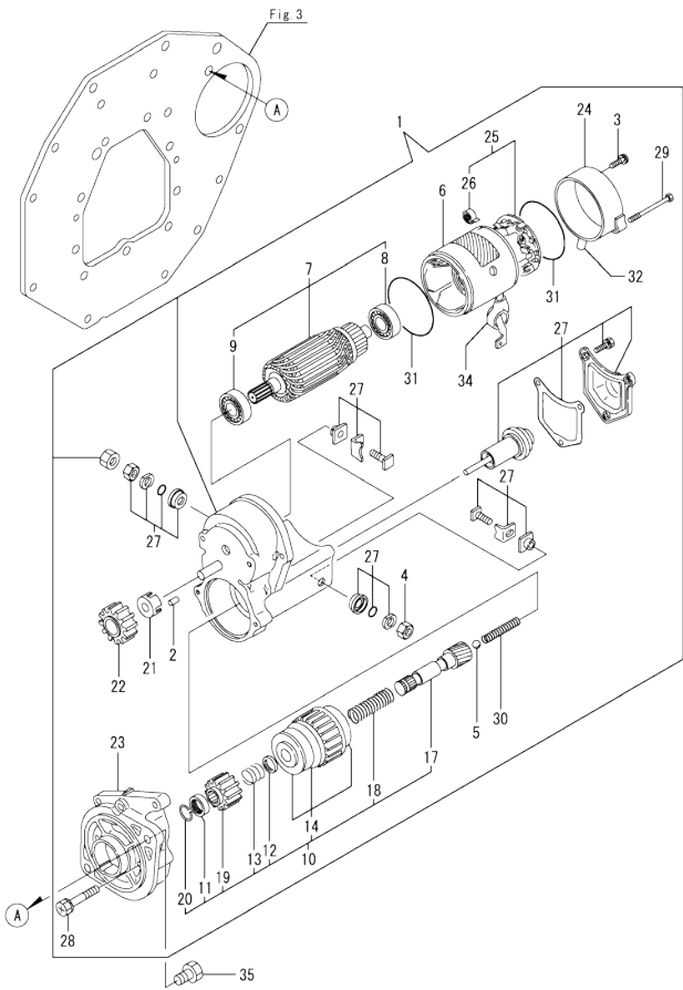
Fig.14. STARTER MOTOR
