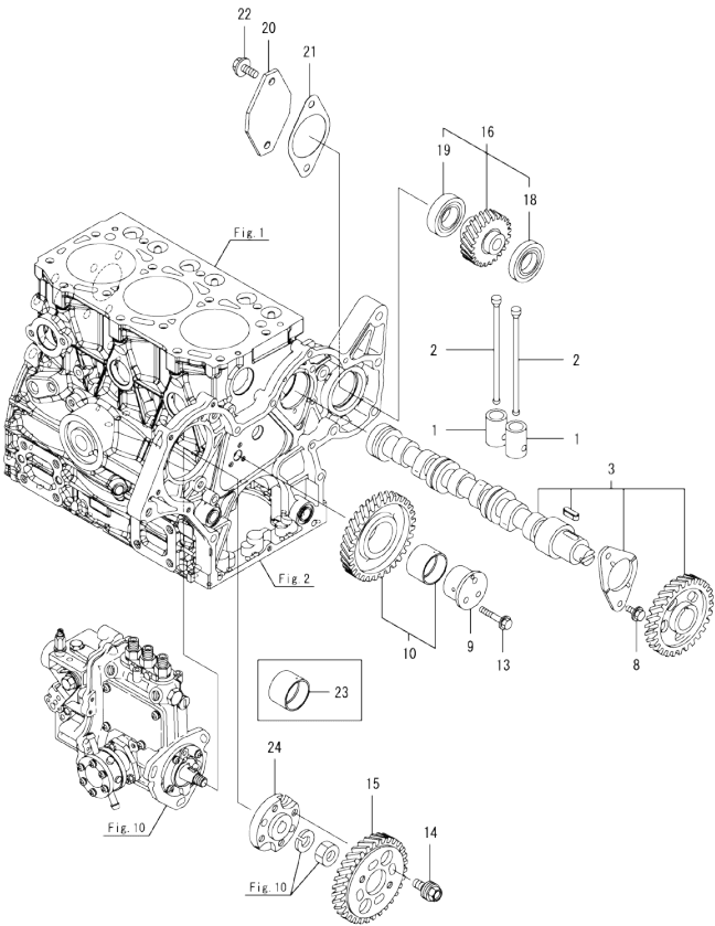
Fig.6. CAMSHAFT & DRIVING GEAR
