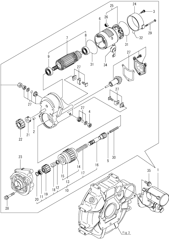
Fig.14. STARTER MOTOR
