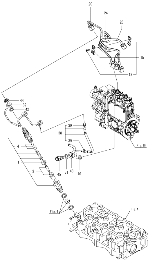
Fig.12. FUEL INJECTION VALVE
