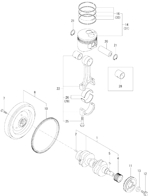
Fig.7. CRANKSHAFT & PISTON
