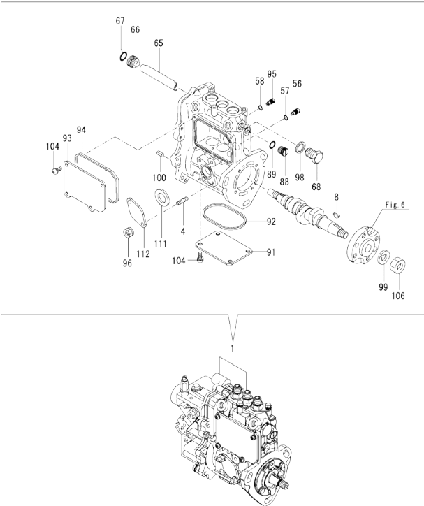
Fig.10. FUEL INJECTION PUMP
