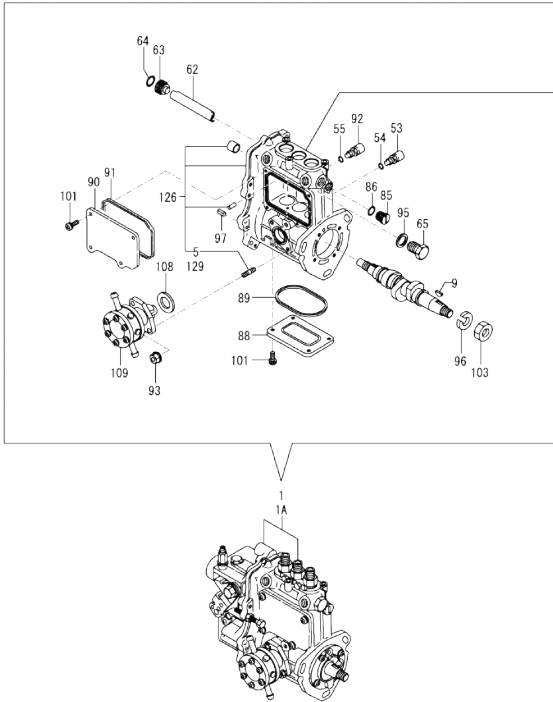
Fig.10. FUEL INJECTION PUMP
