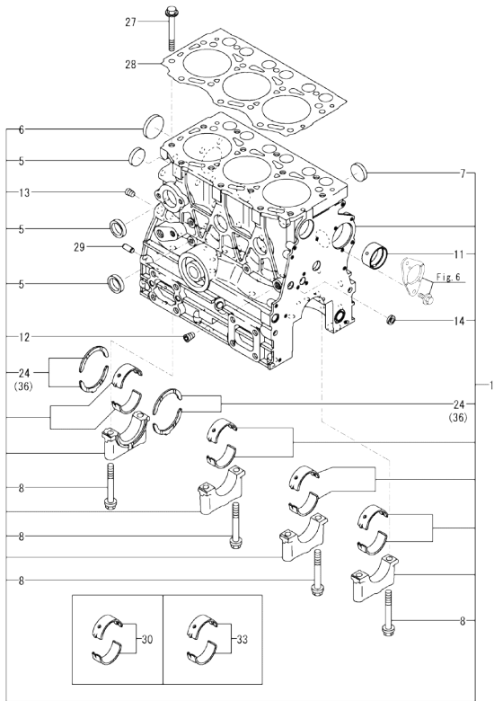
Fig.1. CYLINDER BLOCK
