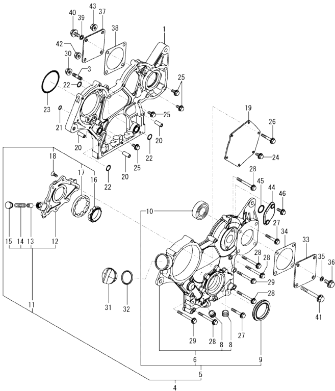
Fig.2. GEAR HOUSING
