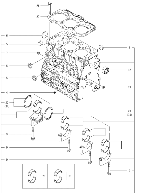
Fig.1. CYLINDER BLOCK
