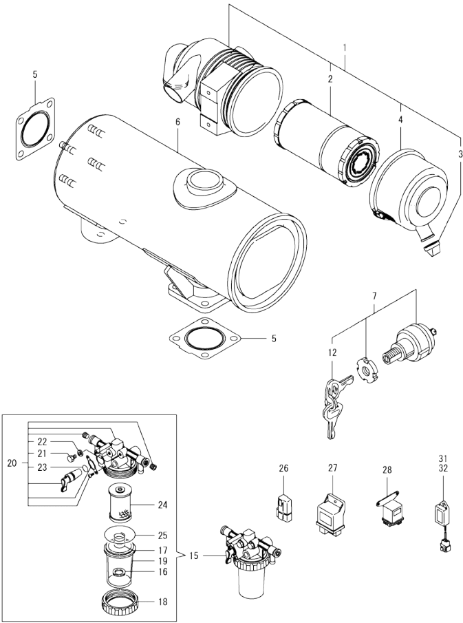
Fig.16. ACCESSORY
