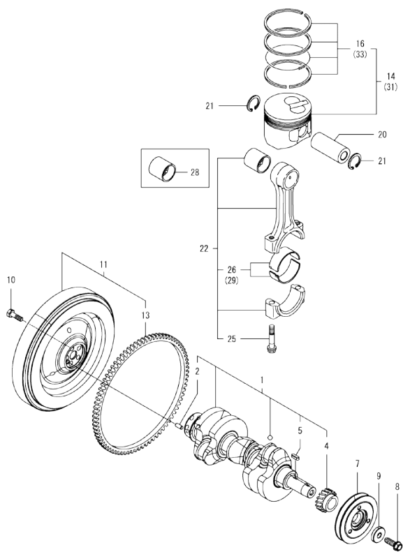
OCD50-M04690 ENGINE Fig.7. CRANKSHAFT & PISTON
