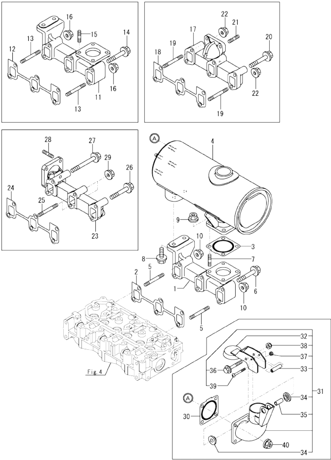
Fig.6. EXHAUST MANIFOLD
