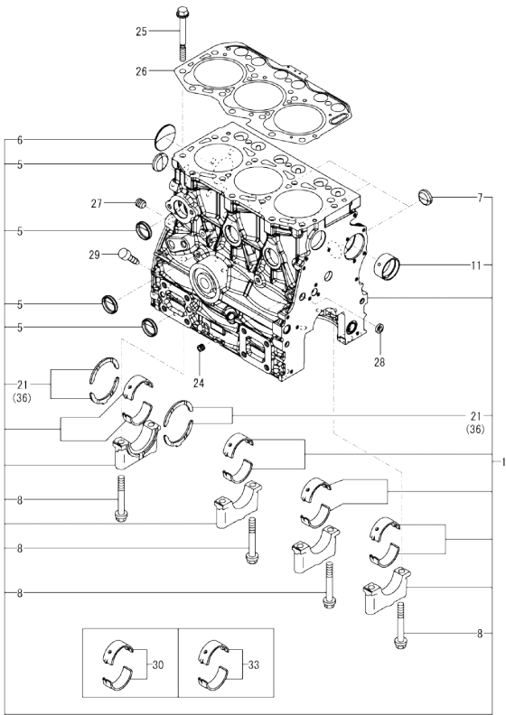
Fig.1. CYLINDER BLOCK
