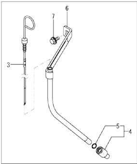
Fig.9. LUB. OIL SYSTEM
