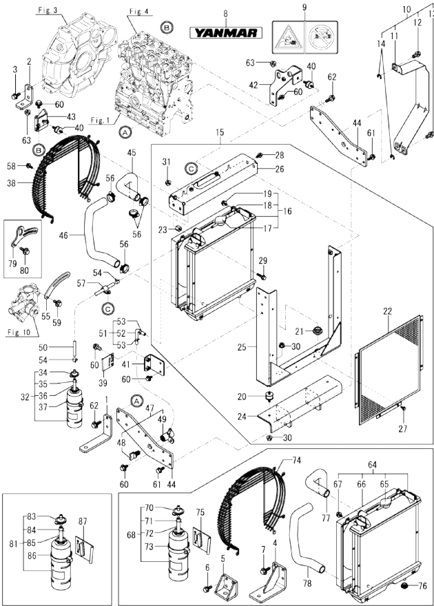
OCD50-M05320 ENGINE Fig.11. RADIATOR
