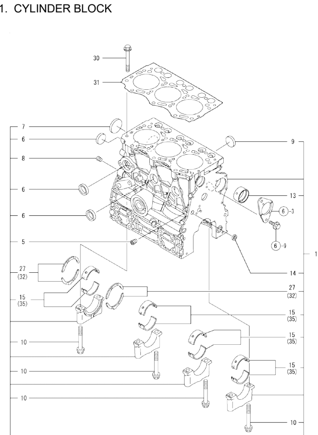
Fig.1. CYLINDER BLOCK
