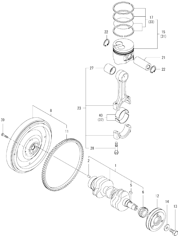
Fig.7. CRANKSHAFT & PISTON
