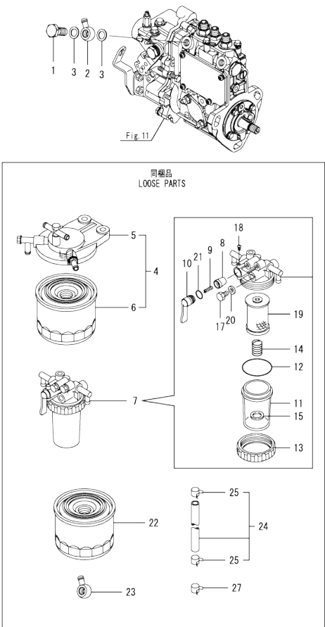
Fig.14. FUEL FILTER
