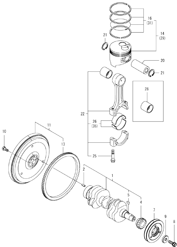
OCD50-M04940 ENGINE Fig.7. CRANKSHAFT & PISTON
