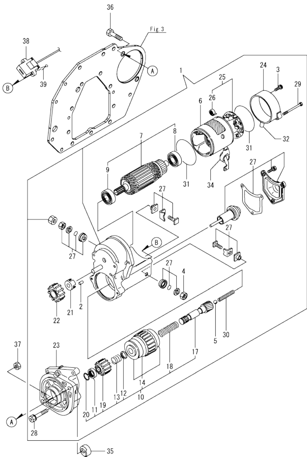
Fig.14. STARTER MOTOR
