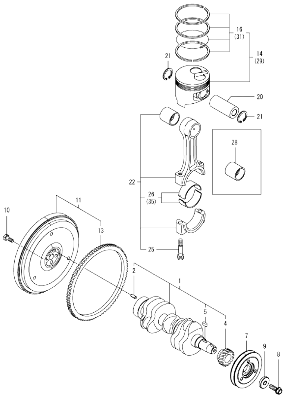
OCD50-M04960 ENGINE Fig.7. CRANKSHAFT & PISTON
