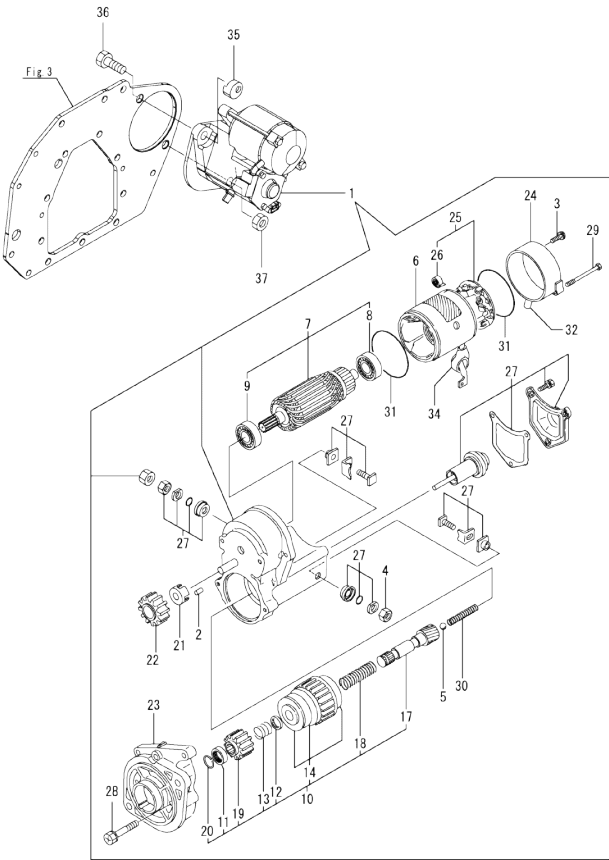
Fig.14. STARTER MOTOR
