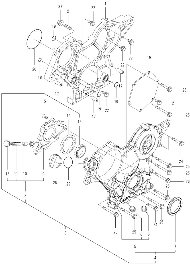
OCD50-M01620 3TNV76-XPND Fig.2. GEAR HOUSING
