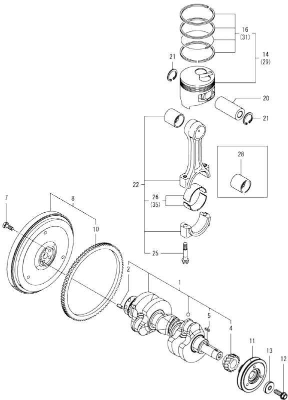
Fig.7. CRANKSHAFT & PISTON
