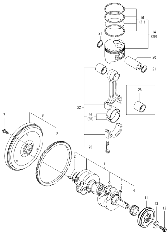
OCD50-M06340 ENGINE Fig.7. CRANKSHAFT & PISTON
