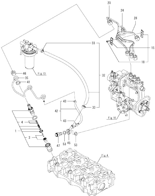
OCD50-M00550 3TNV80F-NGGE Fig.12. FUEL INJECTION VALVE
