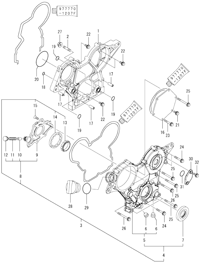
Fig.2. GEAR HOUSING
