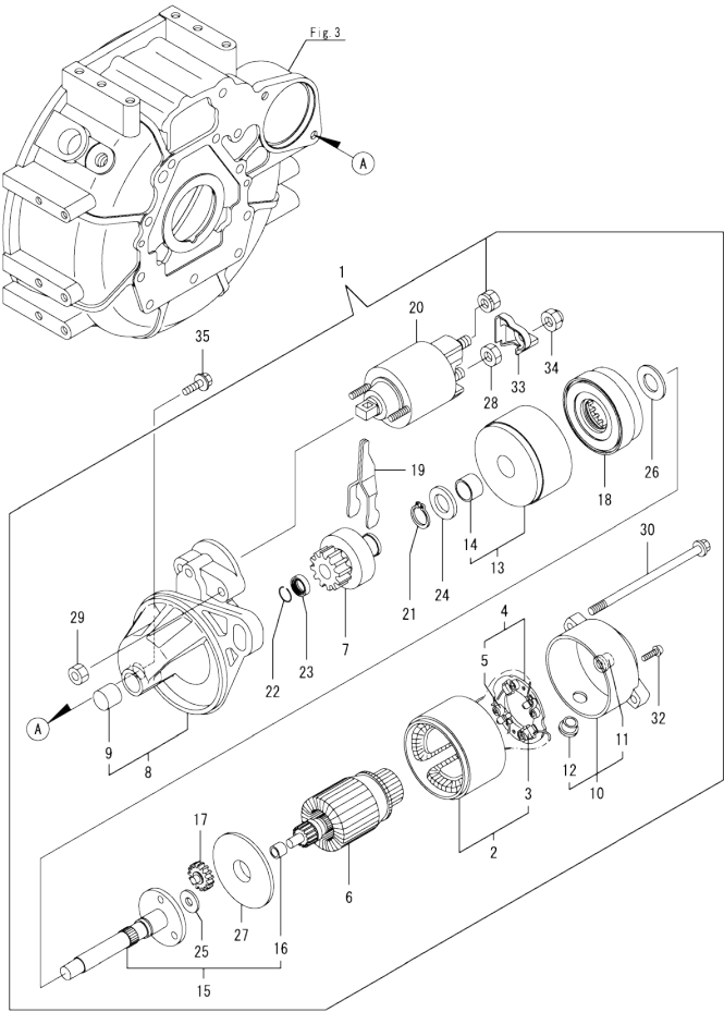
Fig.14. STARTER MOTOR
