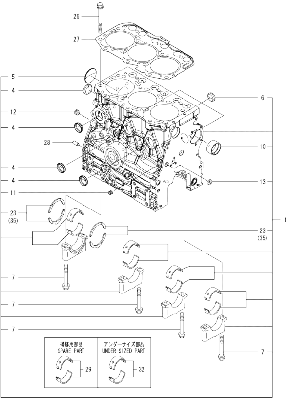
OCD50-M00550 3TNV80F-NGGE Fig.1. CYLINDER BLOCK
