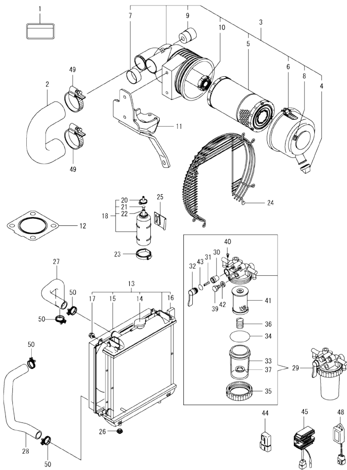
OCD50-M05000 ENGINE Fig.16. ACCESSORY
