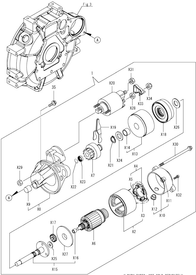
Fig.14. STARTER MOTOR
