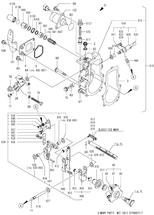
OCD50-M03860 ENGINE Fig.11. GOVERNOR
