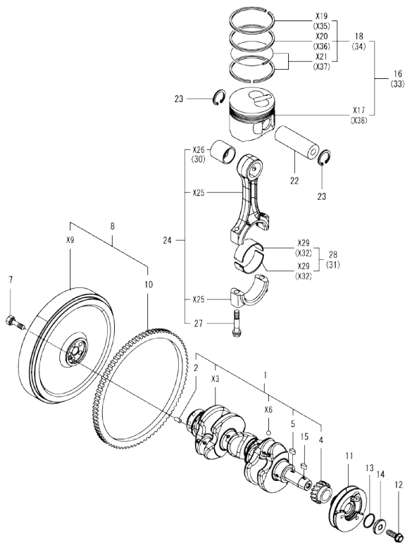
OCD50-M03860 ENGINE Fig.7. CRANKSHAFT & PISTON
