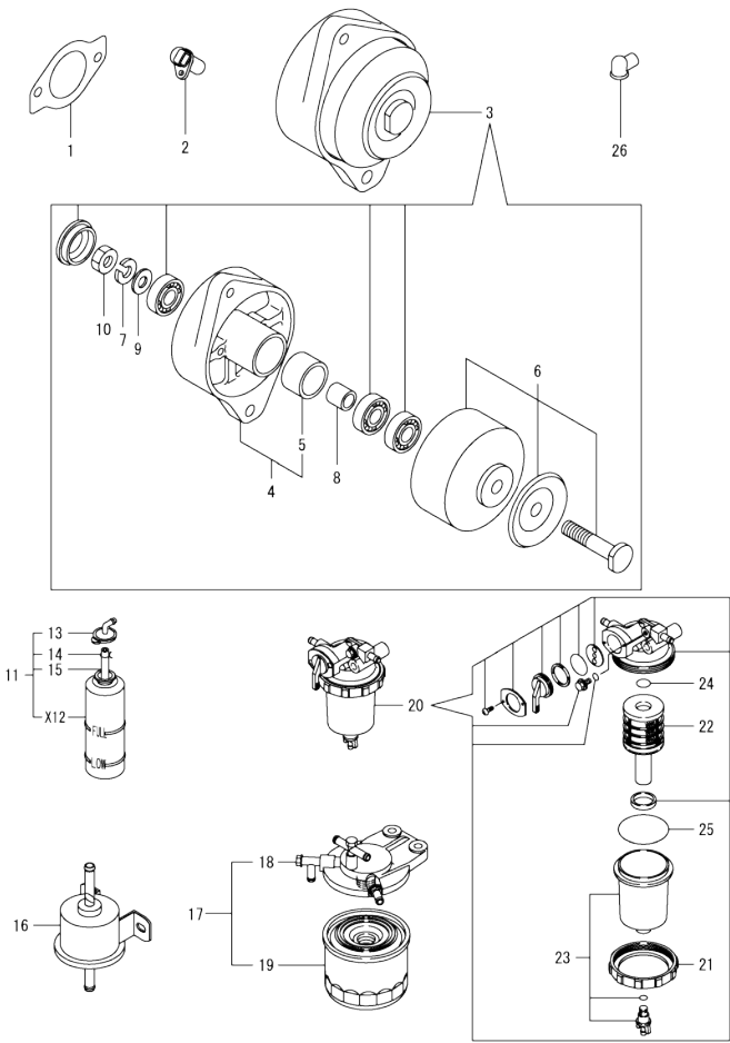
Fig.15. ACCESSORY
