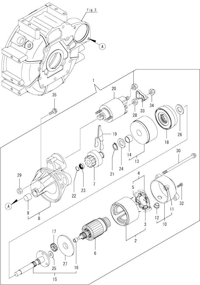
Fig.14. STARTER MOTOR
