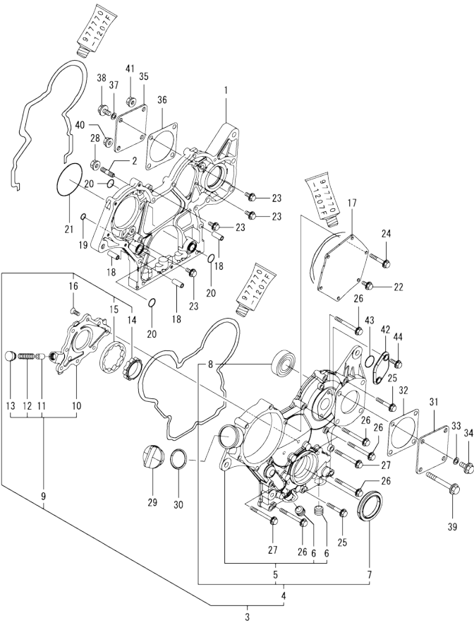
Fig.2. GEAR HOUSING
