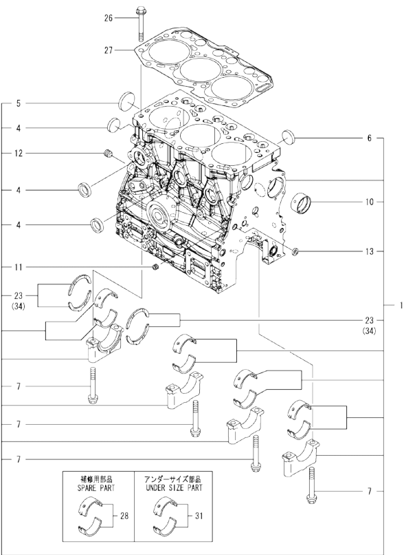
OCD50-M00580 3TNV80F-SDSA Fig.1. CYLINDER BLOCK
