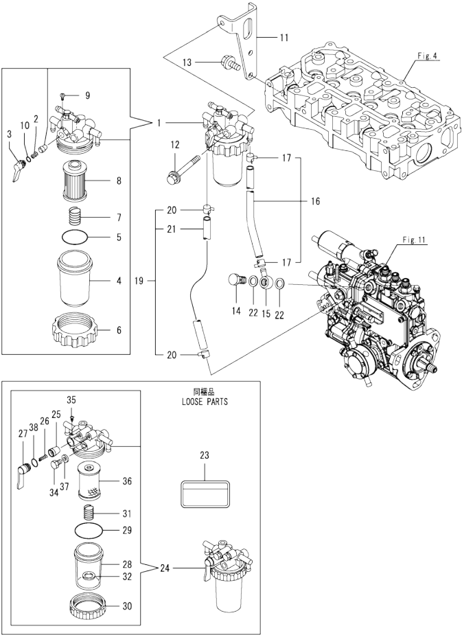
Fig.13. FUEL PIPE
