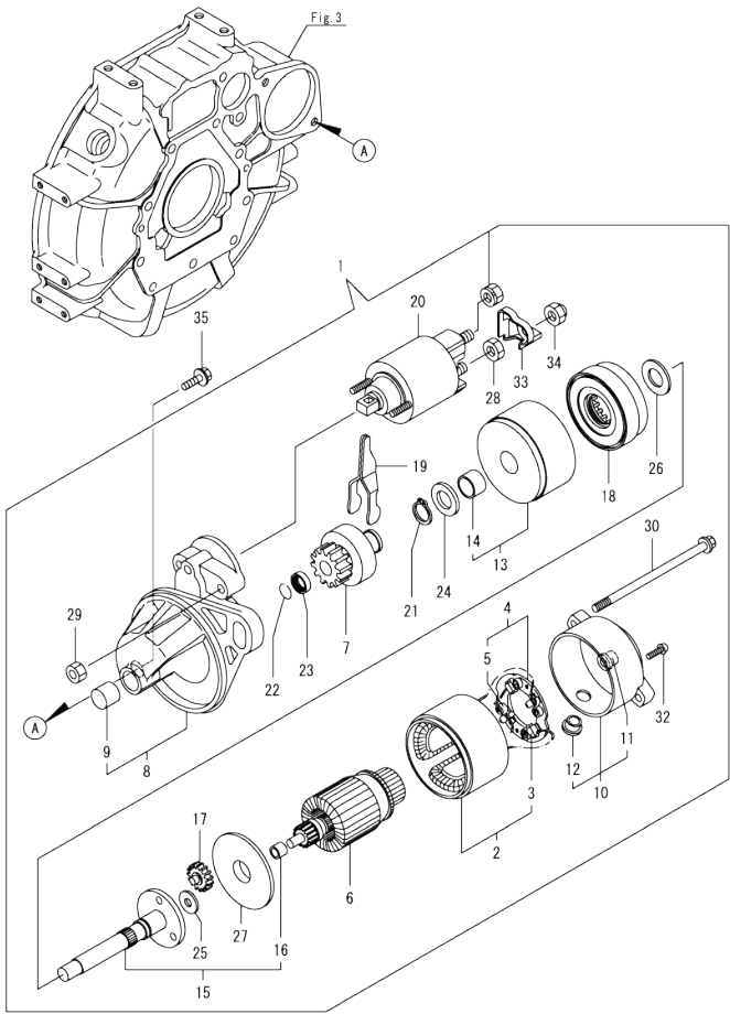
Fig.14. STARTER MOTOR
