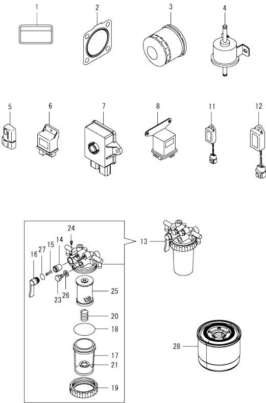
Fig.16. ACCESSORY
