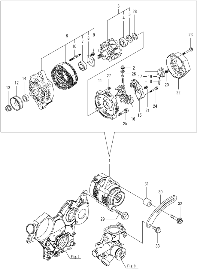
OCD50-M04310 ENGINE Fig.15. GENERATOR
