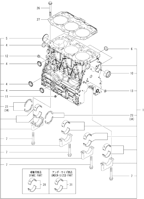
OCD50-M00970 3TNV80F-SNFK Fig.1. CYLINDER BLOCK
