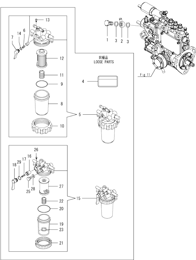
Fig.14. FUEL FILTER
