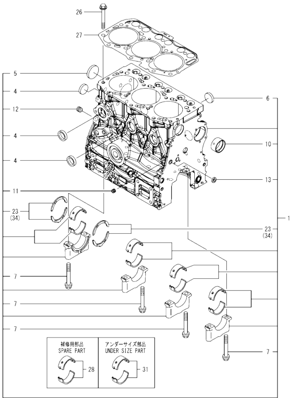
Fig.1. CYLINDER BLOCK
