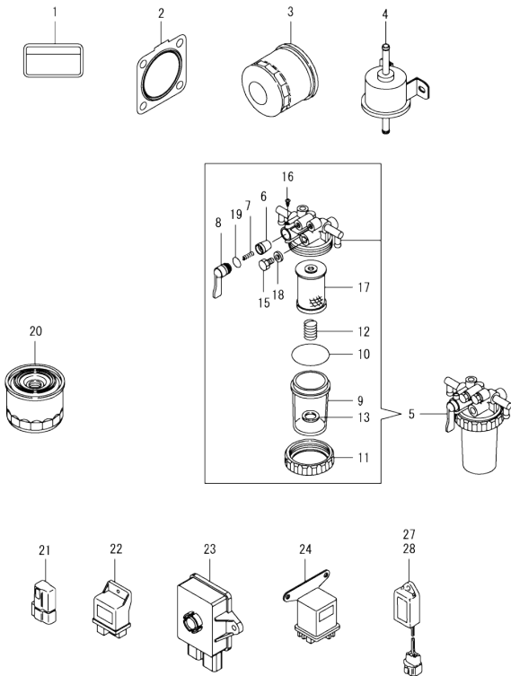
Fig.16. ACCESSORY
