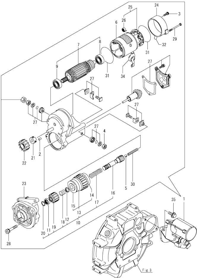
Fig.14. STARTER MOTOR
