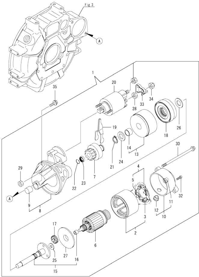
Fig.15. STARTER MOTOR
