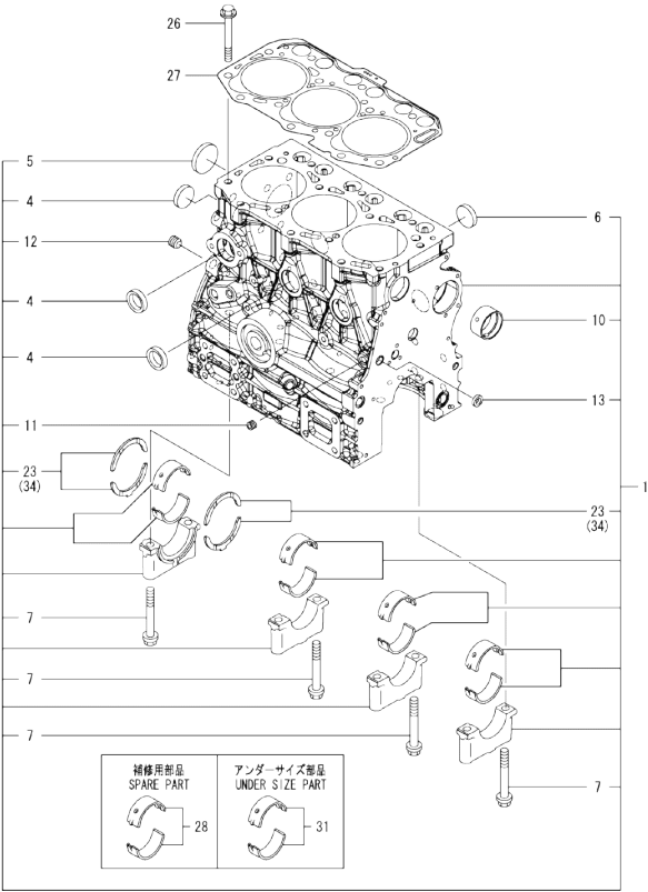
OCD50-M01510 3TNV80F-SNMB Fig.1. CYLINDER BLOCK
