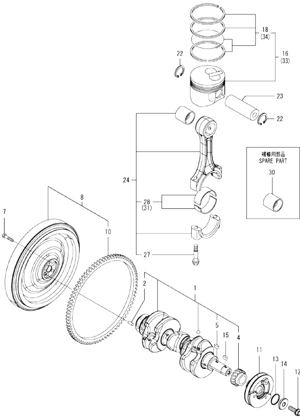
Fig.7. CRANKSHAFT & PISTON
