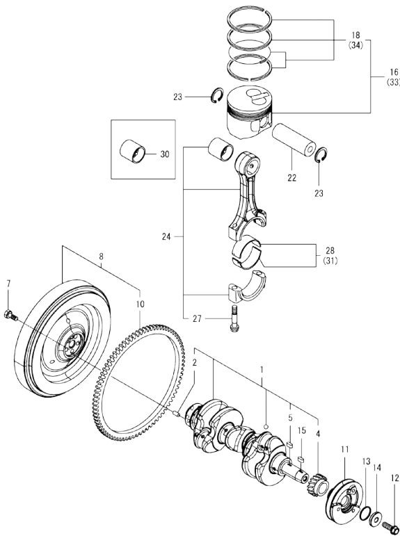
OCD50-M05570 ENGINE Fig.7. CRANKSHAFT & PISTON
