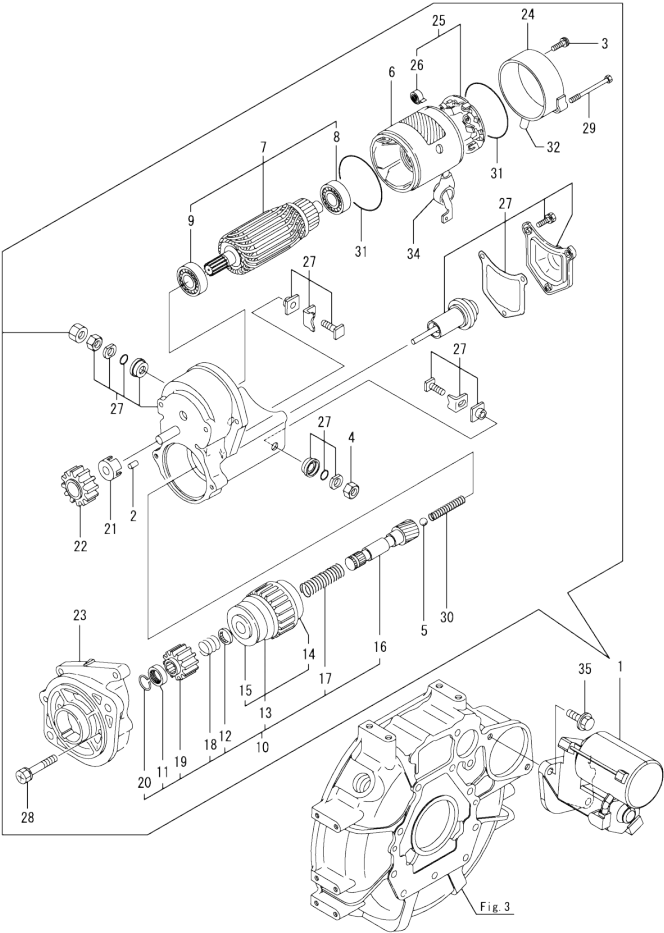
OCD50-M02100 3TNV80F-SPSU Fig.15. STARTER MOTOR
