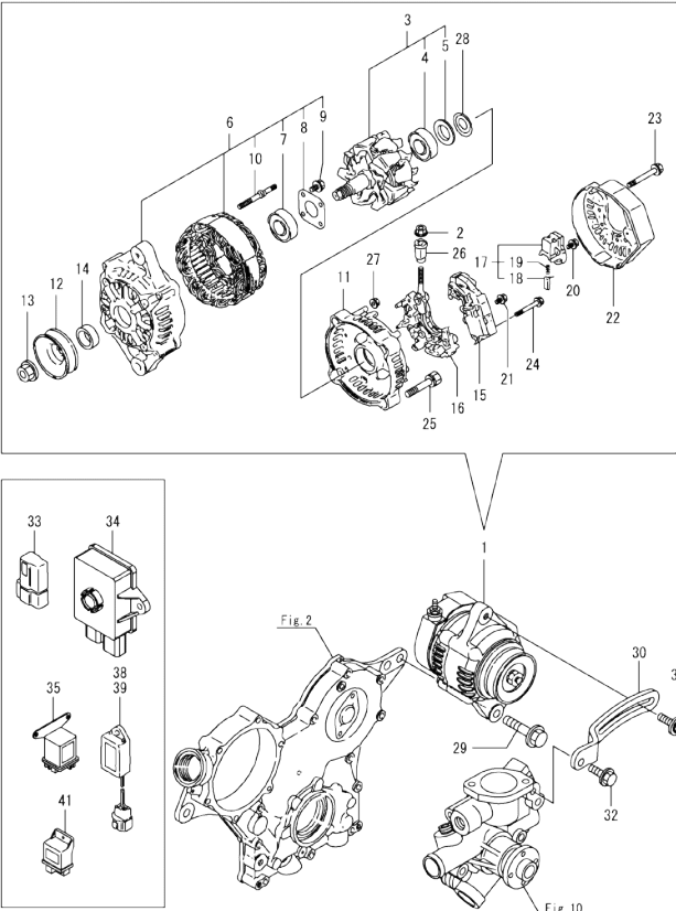
OCD50-M02100 3TNV80F-SPSU Fig.16. GENERATOR
