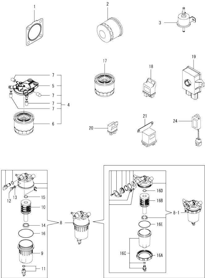
Fig.16. ACCESSORY
