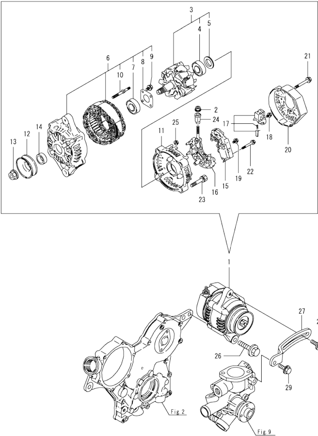
OCD50-M07100 ENGINE Fig.15. GENERATOR
