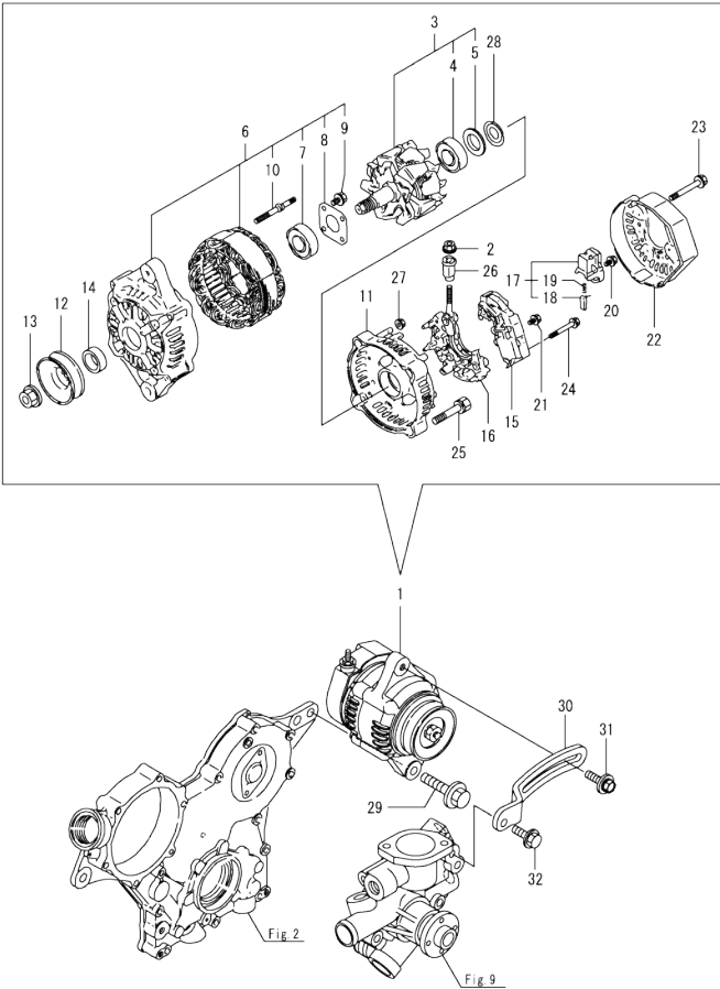
OCD50-M04140 ENGINE Fig.15. GENERATOR
