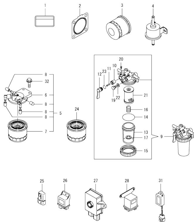
OCD50-M04140 ENGINE Fig.16. ACCESSORY
