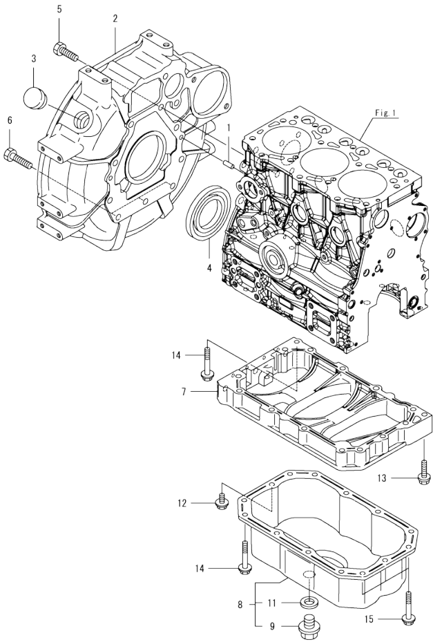
Fig.3. FLYWHEEL HOUSING & OIL SUMP
