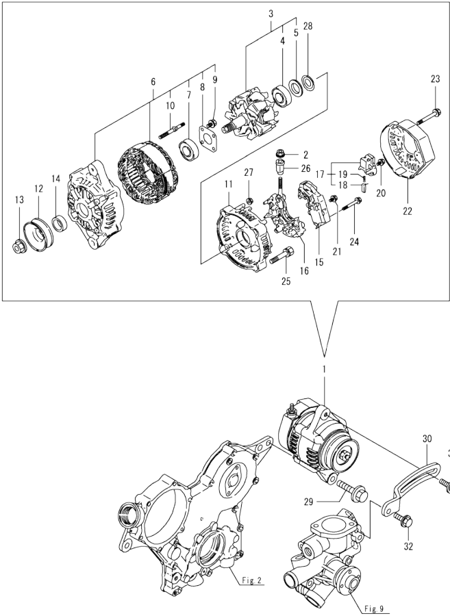
OCD50-M03080 ENGINE Fig.15. GENERATOR
