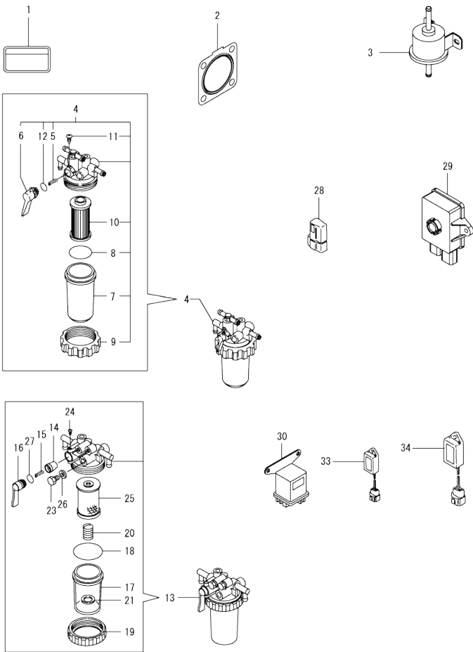
Fig.16. ACCESSORY
