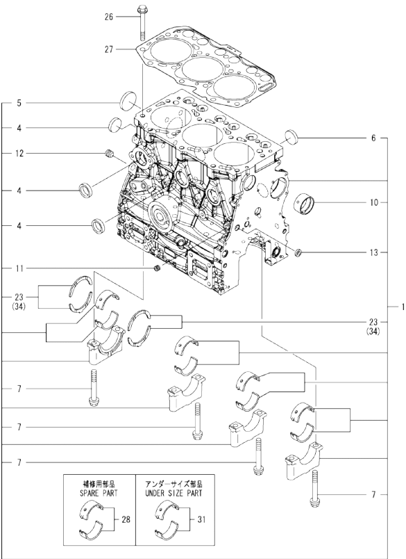
OCD50-M02110 3TNV80F-SSSU Fig.1. CYLINDER BLOCK
