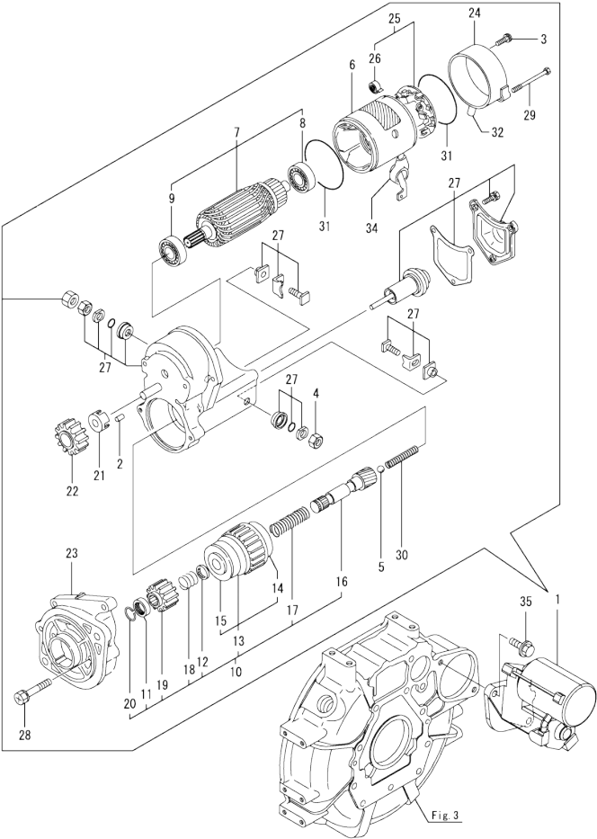
OCD50-M02110 3TNV80F-SSSU Fig.15. STARTER MOTOR
