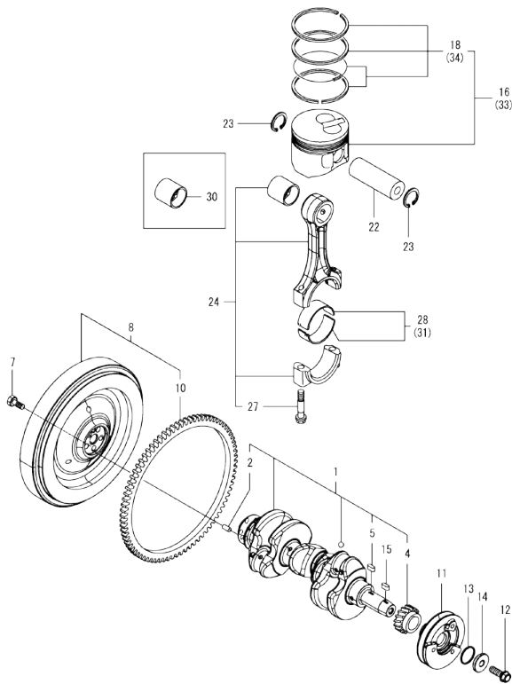
OCD50-M04460 ENGINE Fig.7. CRANKSHAFT & PISTON
