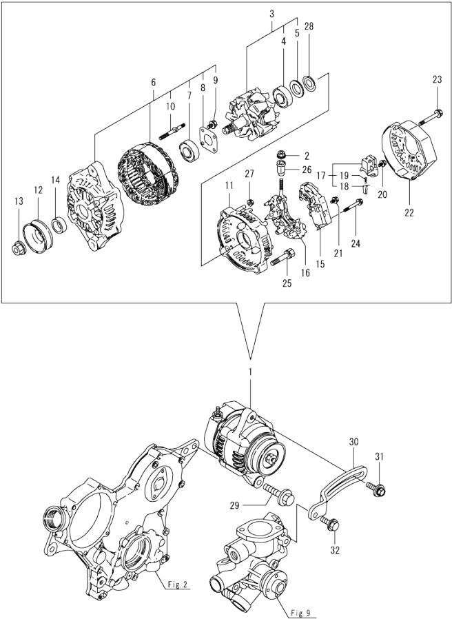
OCD50-M04460 ENGINE Fig.15. GENERATOR
