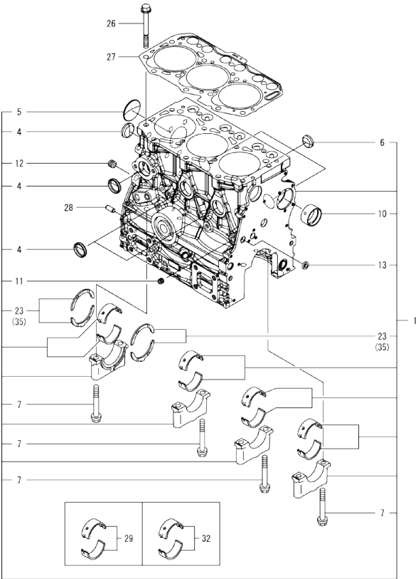
Fig.1. CYLINDER BLOCK
