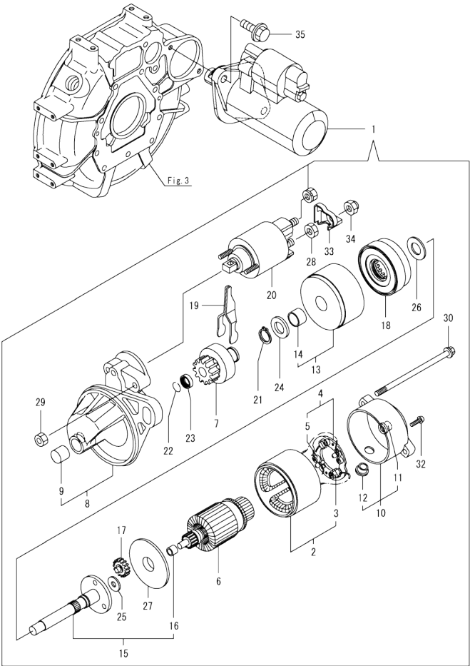
Fig.17. STARTER MOTOR
