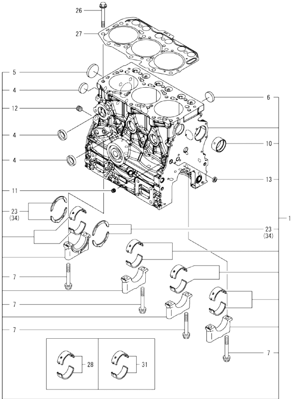
Fig.1. CYLINDER BLOCK
