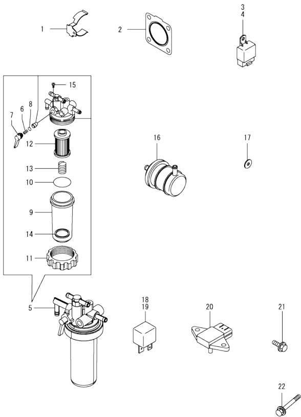
Fig.18. ACCESSORY
