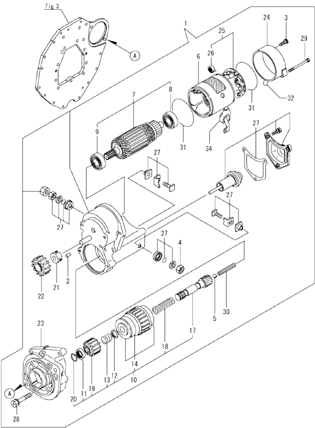
Fig.15. STARTER MOTOR
