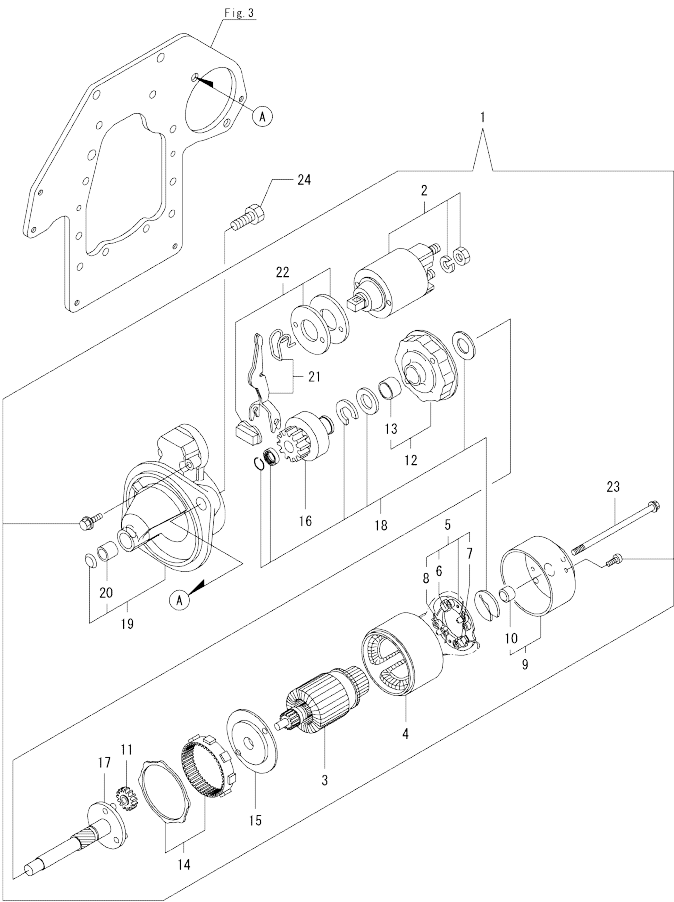
Fig.14. STARTING MOTOR
