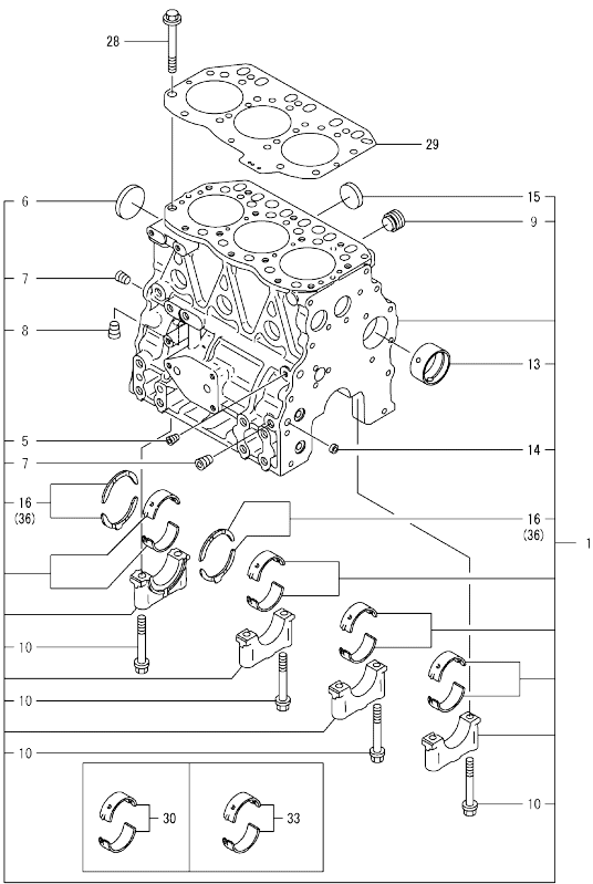
Fig.1. CYLINDER BLOCK
