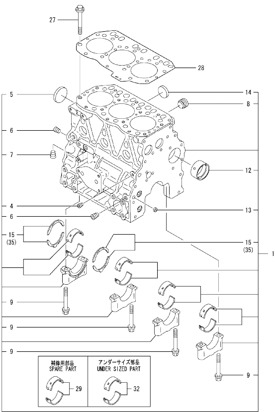
OCD50-M01470 3TNV82A-BDHTR Fig.1. CYLINDER BLOCK
