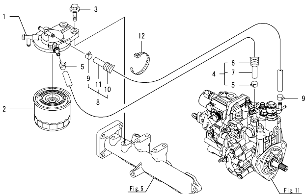
Fig.14. FUEL PIPE
