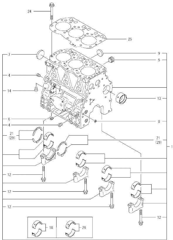
0CW10-M84300 3TNV82A-BDMH Fig.1. CYLINDER BLOCK
