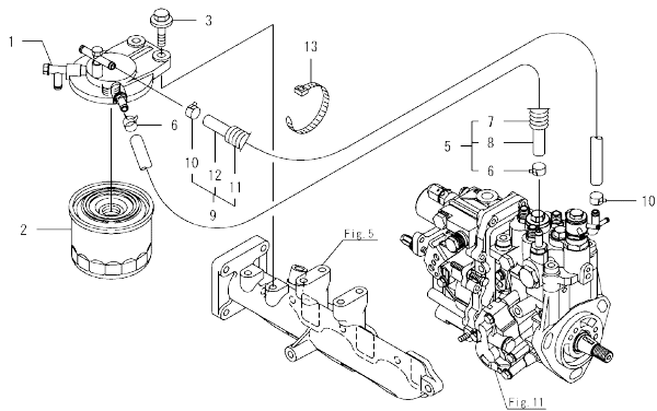
Fig.14. FUEL LINE
