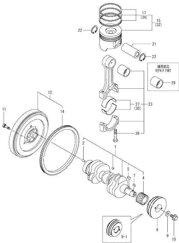
Fig.8. CRANKSHAFT & PISTON
