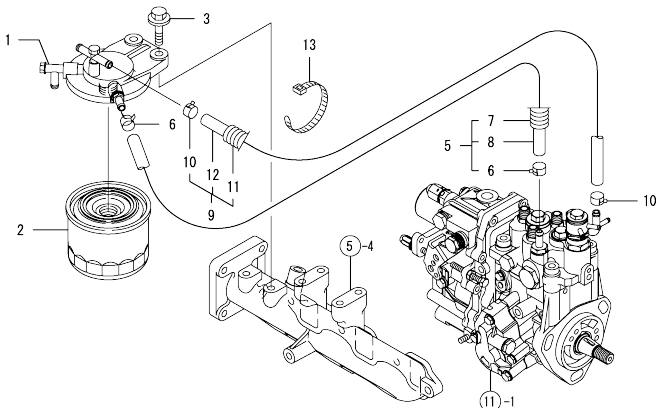
Fig.14. FUEL LINE
