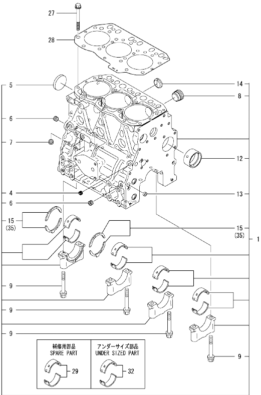
OCD50-M01670 3TNV82A-BDTH Fig.1. CYLINDER BLOCK
