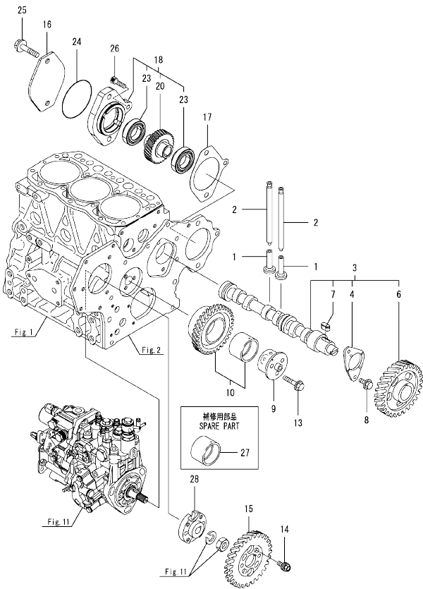
Fig.7. CAMSHAFT & DRIVING GEAR
