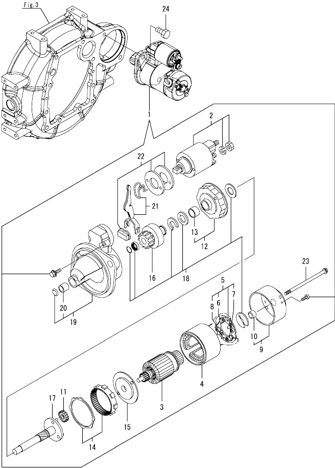
Fig.15. STARTER MOTOR
