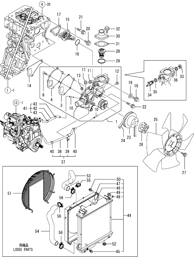
Fig.12. COOLING WATER SYSTEM
