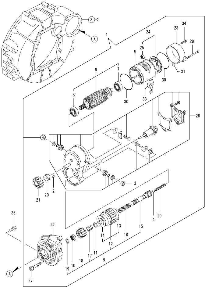
0CW10-M40000 4TNV84T-BGGEH Fig.17. STARTING MOTOR
