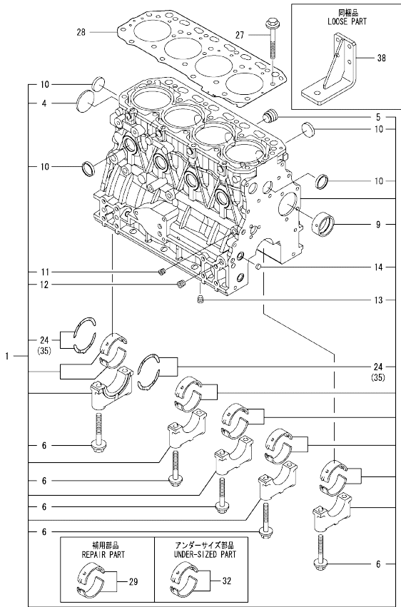
0CW10-M40000 4TNV84T-BGGEH Fig.1. CYLINDER BLOCK
