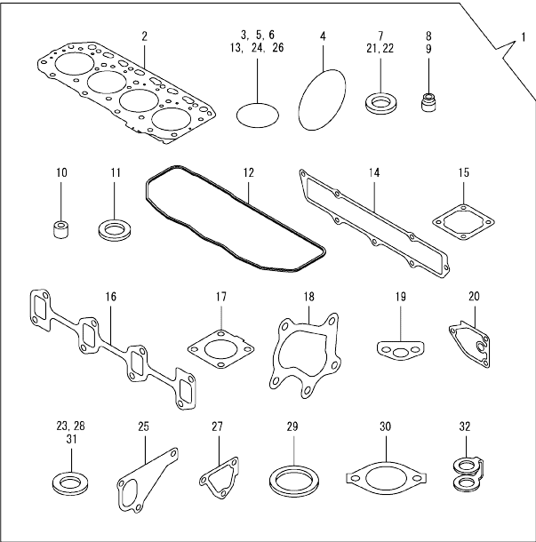
Fig.20. GASKET SET
