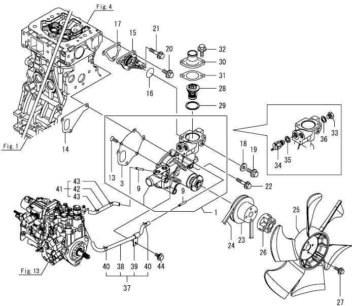
Fig.12. COOLING WATER SYSTEM
