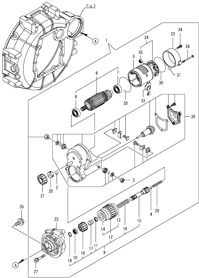
Fig.17. STARTER MOTOR
